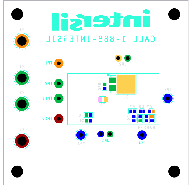
FIGURE 8. SILKSCREEN BOTTOM COMPONENTS
