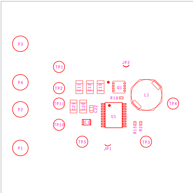
FIGURE 9. TOP COMPONENT ASSEMBLY
